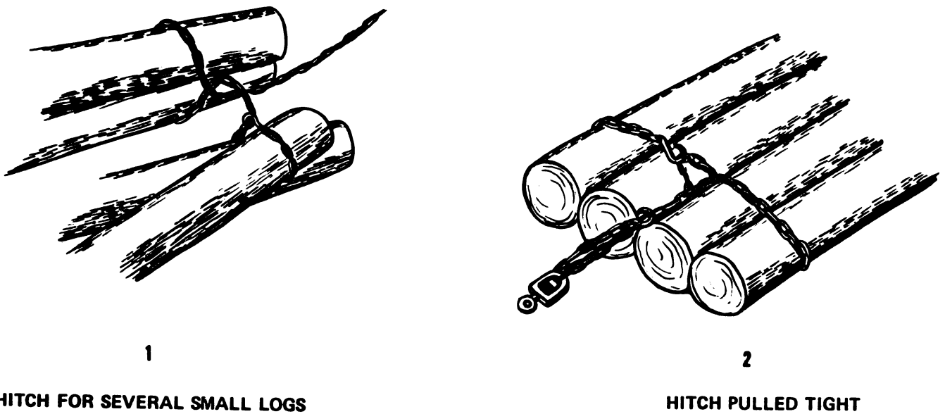
Figure 7-5. Hitch for light logs and poles.
